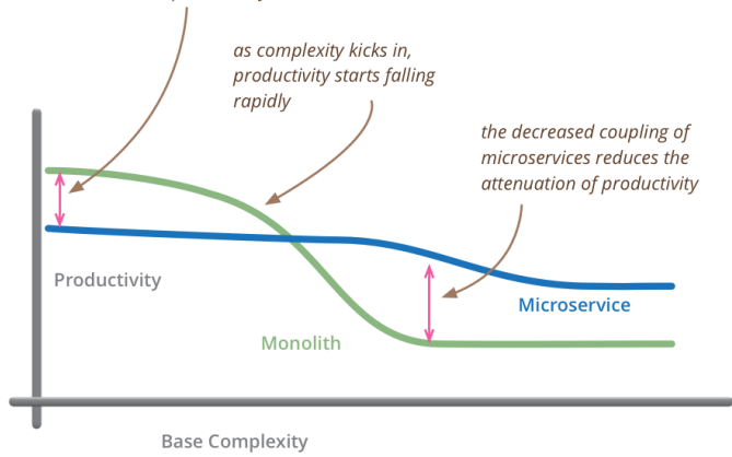
Microservices: productivity versus base complexity (source: Martin Fowler; http://martinfowler.com/bliki/MicroservicePremium.html )
