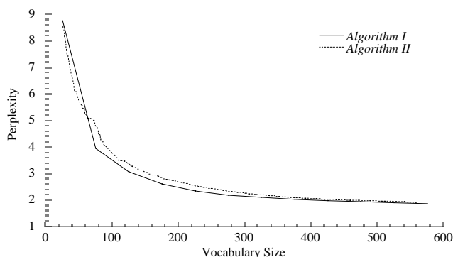
Figure 4. Both algorithms lead to similar results, so the much more economical Greedy strategy demonstrates to be good enough to our purposes.
