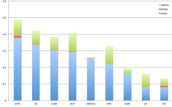
Fig. 3. ATWV, MTWV and UBTWV results on eval queries for primary systems with positive ATWV scores
